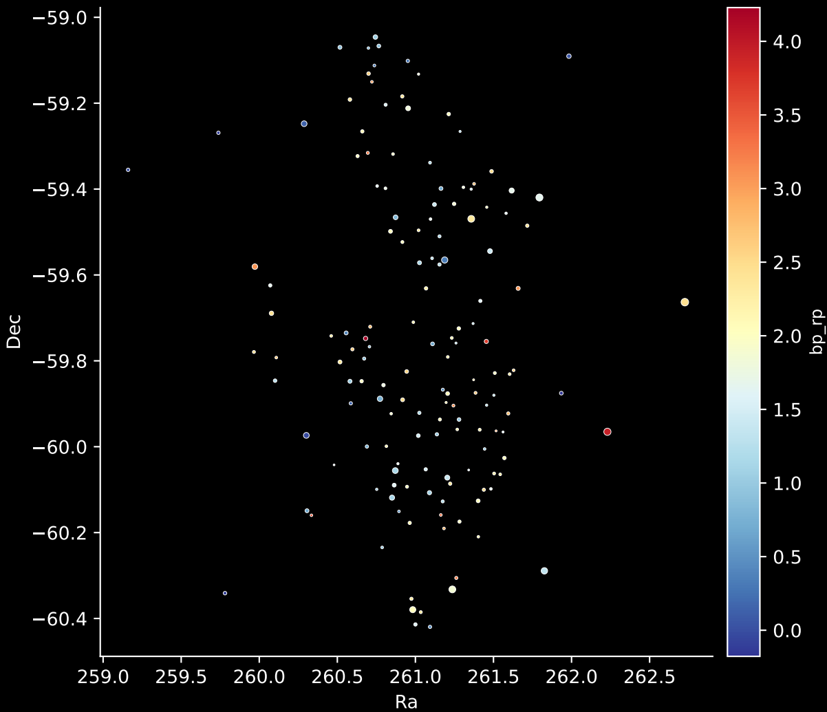
APOGEE DR17 Field: [160-60-C] Stars: 148
