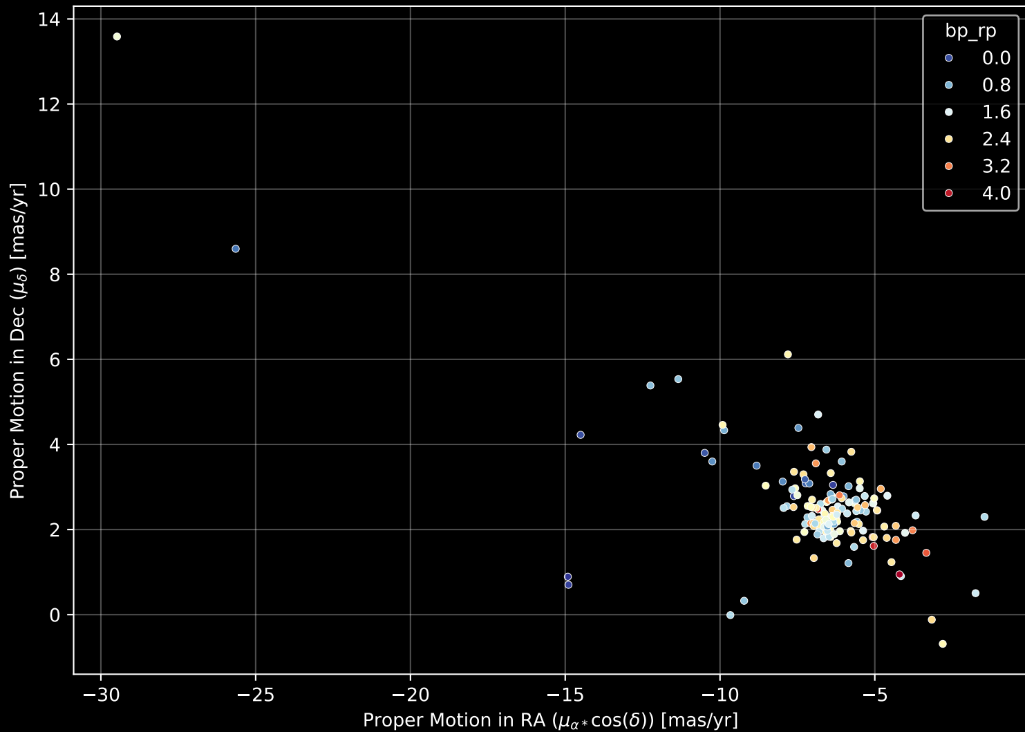
APOGEE DR17 Field: [160-60-C] Proper Motion Diagram (n= 148)
