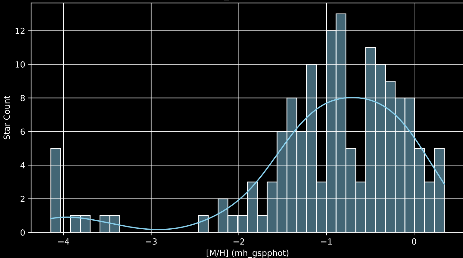
APOGEE DR17 Field: [160-60-C [M/H] (mh_gspphot) (n= 146)
