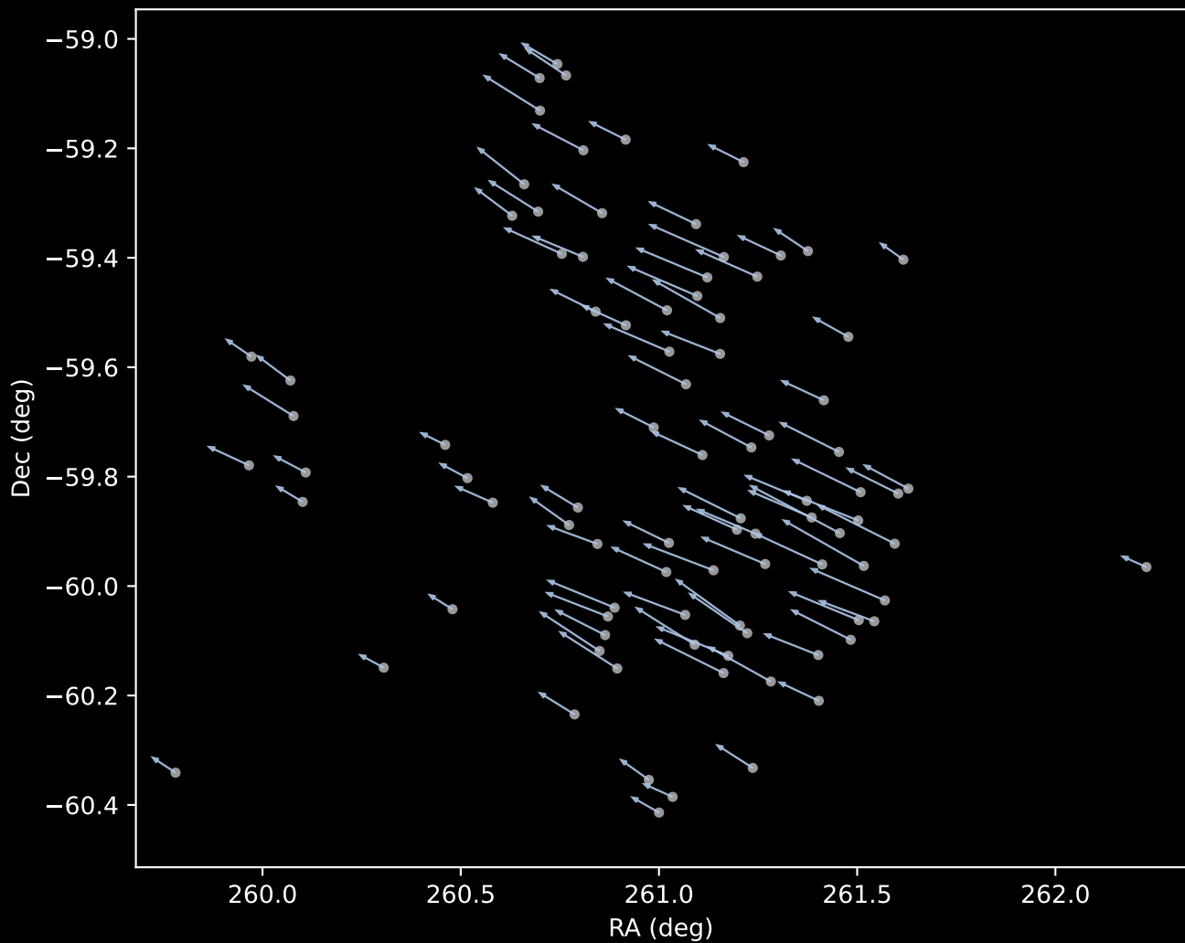
APOGEE DR17 Cluster 1 Proper Motion Vectors (n=91)
