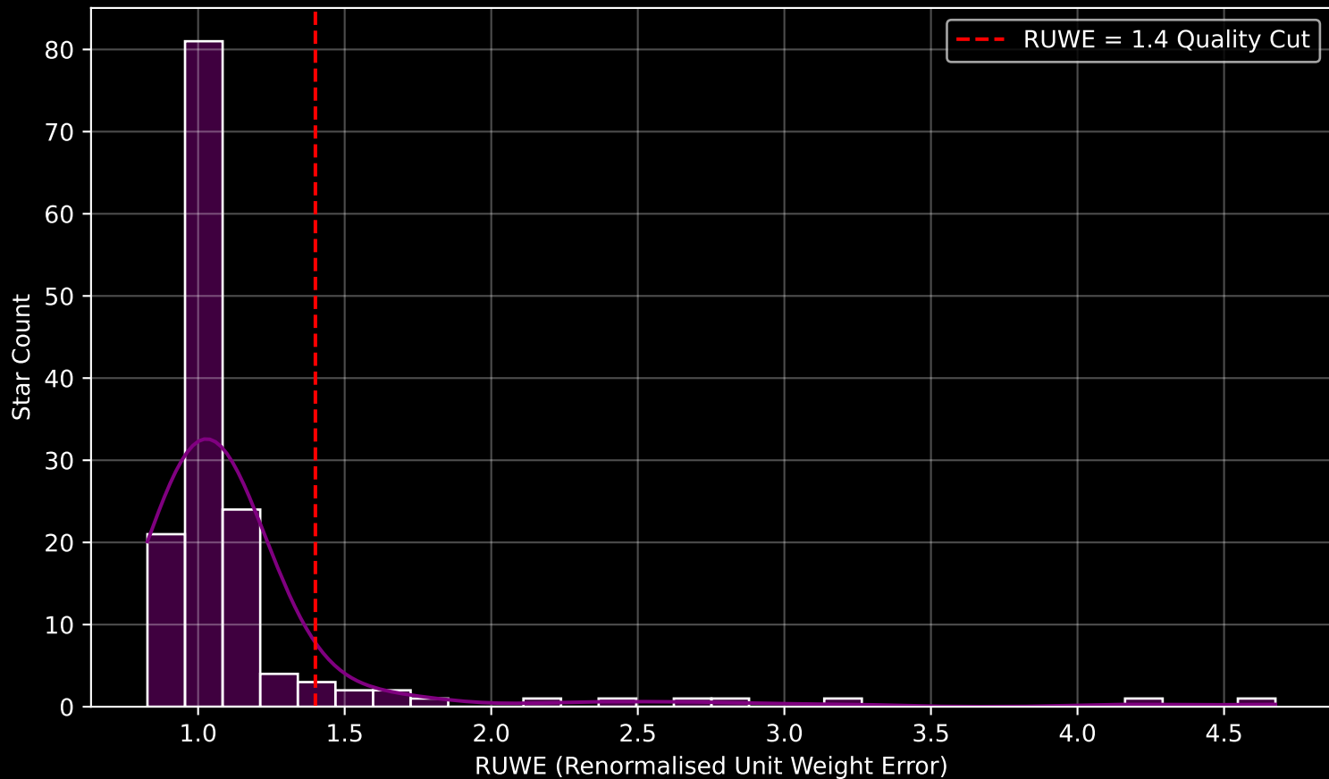
GAPOGEE DR17 Field [160-60-C] RUWE Distribution (n= 145)
