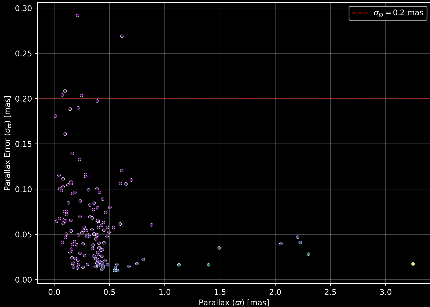
APOGEE DR17 Field: [160-60-C] Parallax Quality (n= 148)
