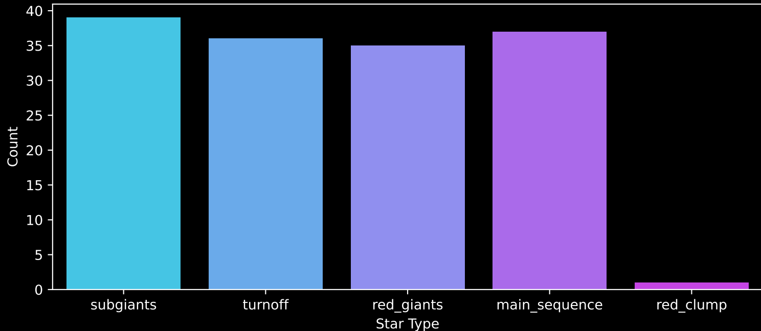
APOGEE DR17 Field: [160-60-C] Count plot of Star Type
